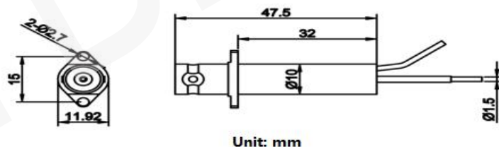
(CSD005A/B, CSD01A/B, CSD02A/B 机械规格)
