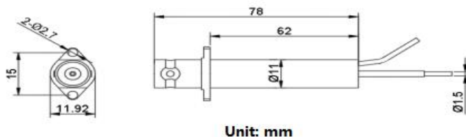
(CSD050A/B, CSD100A/B 机械规格)
